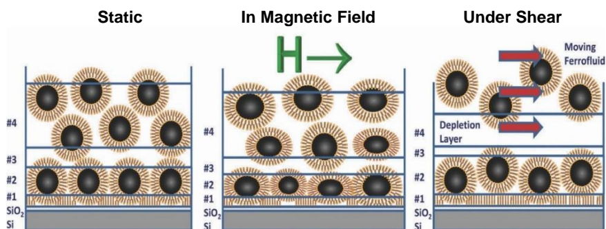
Fig. 9. Models for the layering of the nanoparticles close to the silicon surface. The particles form a densely packed wetting layer at the surface which consists of layer #1 which mostly is ligand material, a densely packed layer #2 containing the cores and ligands between them and a layer #3 which contains ligands and some core material. All layers contain \text{D}_2\text{O}/\text{H}_2\text{O} in addition. Layer #4 is the transition region between the wetting layer and the bulk of the ferrofluid which is not as densely packed as the wetting layer. ( left ) In the static case spherical shaped particles are assumed, ( middle ) in case of an applied field elliptical shaped particles aligned with their long axes in field direction parallel to the silicon surface are assumed, and ( right ) under shear a depletion layer was found between the wetting layer and the moving ferrofluid
