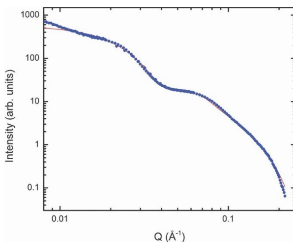
Fig. 3. Educued SANS data taken from a similar ferrofluid and fit to a core–shell model
