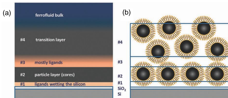
Fig. 5. Model of layers for the superstructure which was assumed for performing fits to the reflectivity data. Schematic layer model (a) and hypothetical particle ordering within the layers #1–4 (b)
