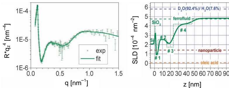
Fig. 6. NR data taken in static conditions without applying a magnetic field. (left) Plot of Rq_z^4 as function of qz . The solid lines represent fits to the data. (right) Profile of nuclear scattering length density plotted as function of distance from the Si (100) surface determined from results of the least square fitting routines applied to the reflectivity data
