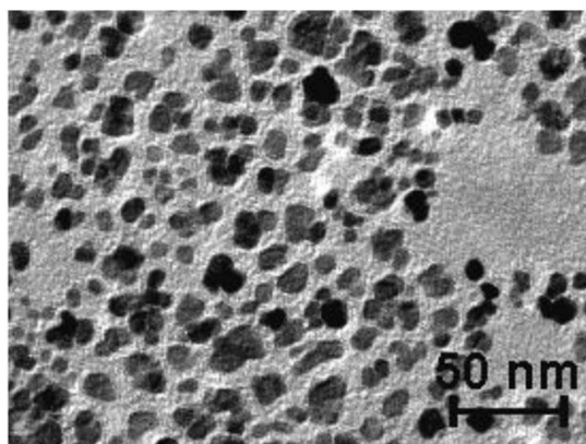
Fig. 2. TEM image taken from the magnetite nanoparticles
