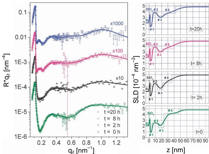
Fig. 8. NR data taken before (green symbols) and during applying a magnetic field of 11 mT parallel to the Si(100) for 2 h (black symbols), 8 h (pink symbols) and after 20 h (blue symbols). (left) Plot of Rq_z^4 as function of q_z . The solid lines represent fits to the data. (right) Profile of nuclear scattering length densities plotted as function of distance from the Si(100) surface determined from results of the least square fitting routines applied to the reflectivity curves
