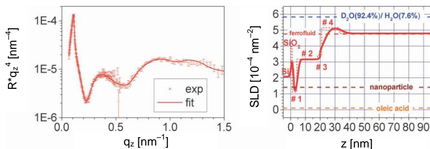
Fig. 10. NR data taken under shear without applying a magnetic field. The fluid was pumped through the flow cell with a volumetric flow rate of Q = 1000 \text{ ml min}^{-1} corresponding to a shear rate of \dot{\gamma} = 313 \text{ s}^{-1} . The solid lines represent fits to the data. ( right ) Profile of nuclear scattering length density plotted as function of distance from the Si(100) surface determined from results of the least square fitting routines applied to the reflectivity curves
